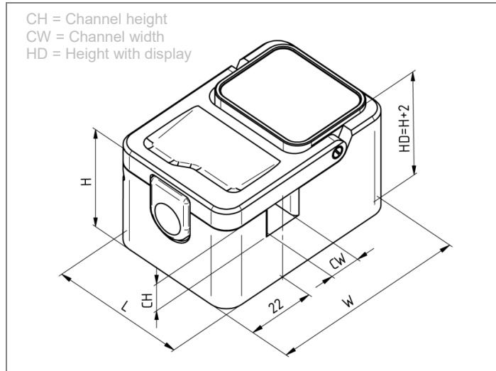
Figure 1: Dimensions SONOFLOW CO.55/xxxSD V2.0
