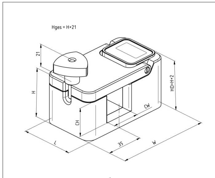
Figure 3: Dimensions SONOFLOW CO.55/xxxSDH V2.0
